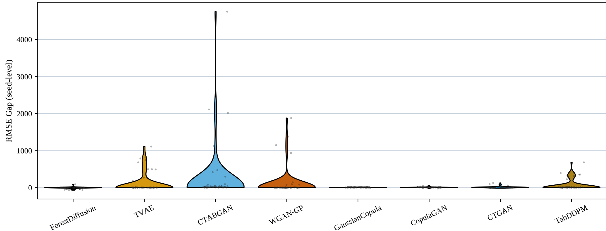
RMSE Gap — seed-level distribution (n = 10 seeds × datasets)
